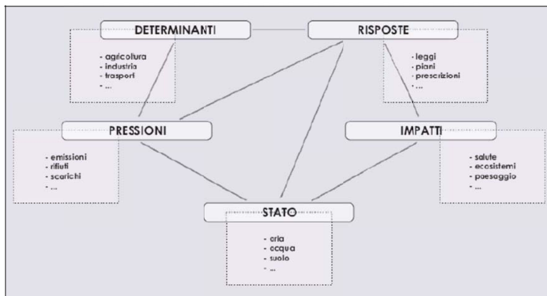
Figura 2.1 – Schema DPSIR
